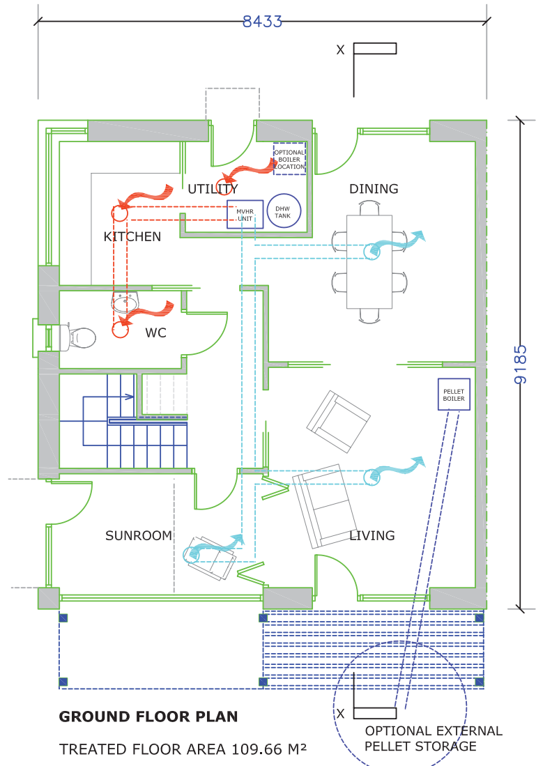
Prototype passive house, floor plans (not to scale). Source: MosArt Architecture
